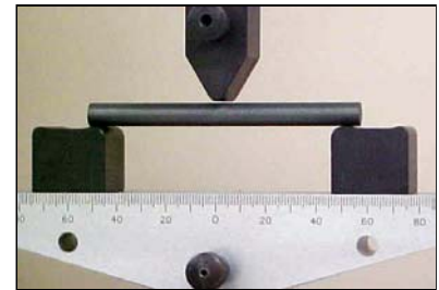
TestResources G238 Bend Fixtures testing ferrite rods.
