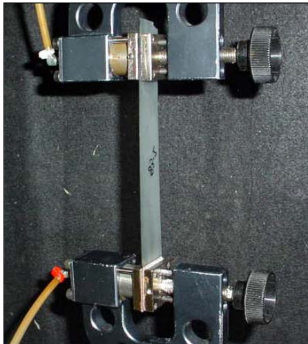
TestResources G94 Lightweight Air Grips performing tensile tests on thin film.
