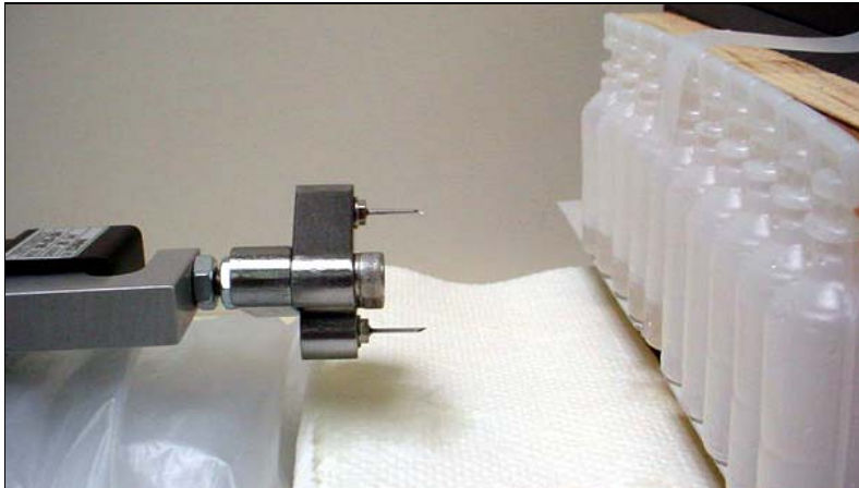
TestResources 200R Test System mounted horizontally to perform needle puncture tests on bottles used in medical applications.
