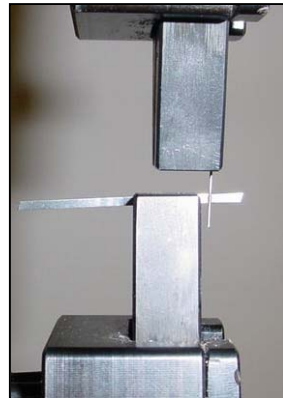
TestResources G7W Wedge Action Grips perform low force fatigue tests on welds and solder joints.
