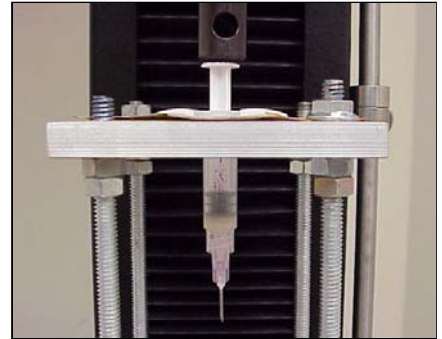
Syringe Test tested using a TestResources 200R Test System
