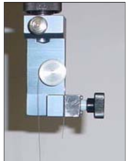
TestResources G76-1 Fine Wire Capstan Grips perform strength tests on small diameter wires common to medical devices.
